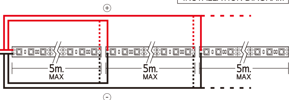
INSTALLATION DIAGRAM
