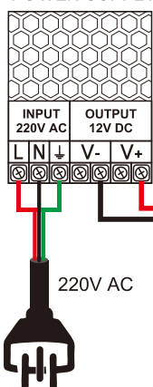
POWER SUPPLY
